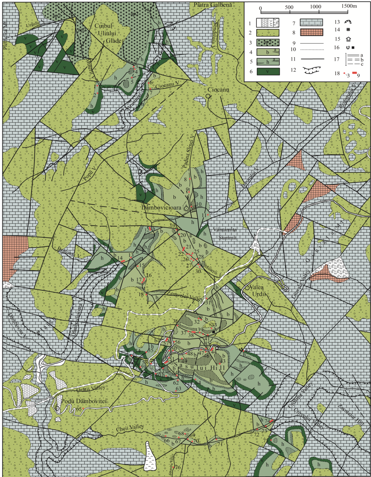
Fig. 1 Geological Map of the Dâmbovicioara Region. Legend: 1, Quaternary (alluvial deposits, terraces, gravelites); 2, the Podu Dâmbovitei Sandstone (Upper Albian); the Gura Văii Conglomerate (Upper Aptian); 4-6, the Dâmbovicioara Formation: 4*), Valea Muierii Member (uppermost Hauterivian-lowermost Aptian); 5*), Dealul Sasului Member (uppermost Valanginian-Upper Hauterivian); 6, Cetatea Neamțului Member (Upper Valanginian); 7, the Upper Bajocian-Berriasian-? Lower Valanginian deposits; 8, Crystalline basement; 9, boundary of the Quaternary deposits; 10, lithostratigraphic boundary; 11, fault; 12, gorge; 13, cave; 14 ruins of the "Neamțului" fortress; 15, the "Dealul Sasului" Inn; 16, winter-stable, sheep-fold; 17, routes: a, the Bran-Rucăr highway; b, the old comercial route between Vallachia and Transylvania; c, forest roads and paths (noted when necessary for the location of the sites); 18, fossiliferous sites.
